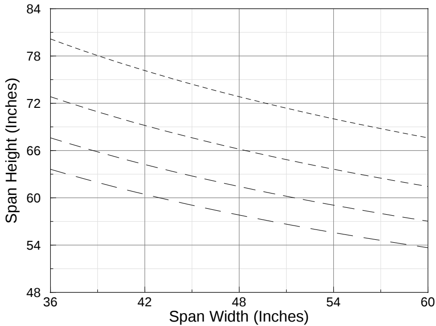
Windload Chart for 7115/6024 Meeting Rail
