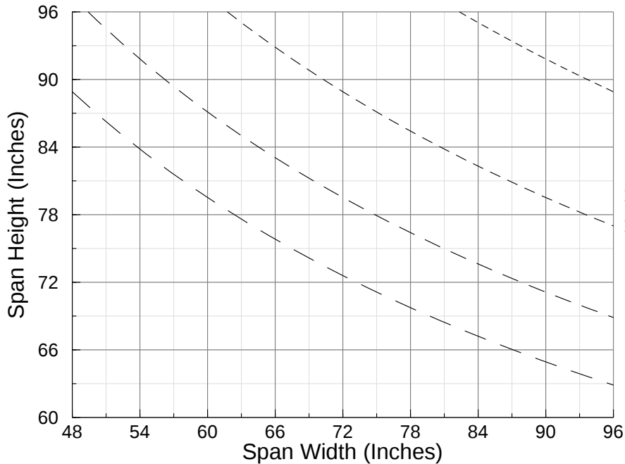
Windload Chart for #6002/7090/6003 I Beam Mullion
